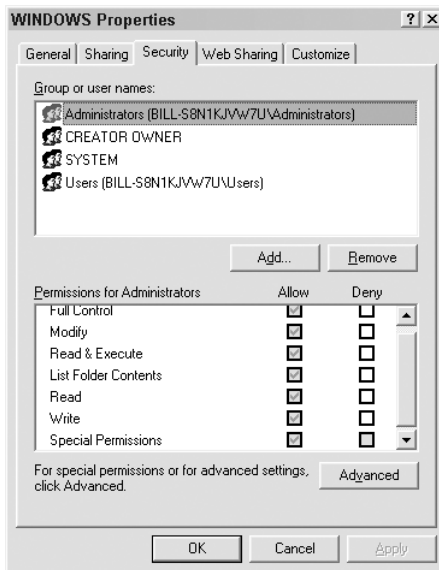
Figure 6.2 Windows file permission granularity.
